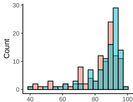
Percentage of Bistable Posterior Draws
