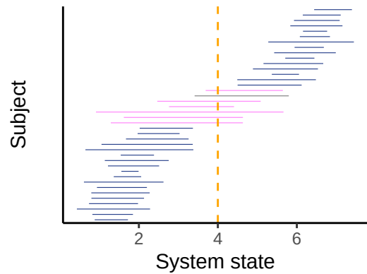
Short time series
